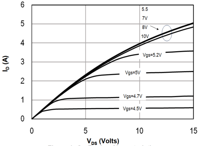
Figure 1: On-Region Characteristics
