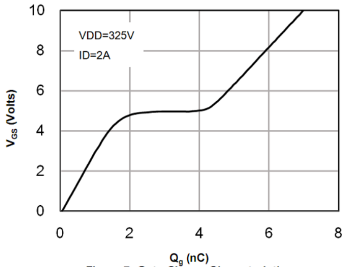
Figure 7: Gate-Charge Characteristics
