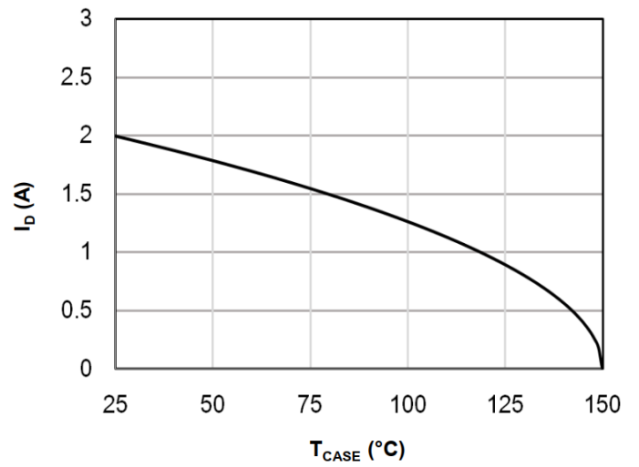
Figure 10: Tcase Temperature
