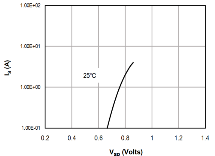
Figure 6: Body-Diode Characteristics
