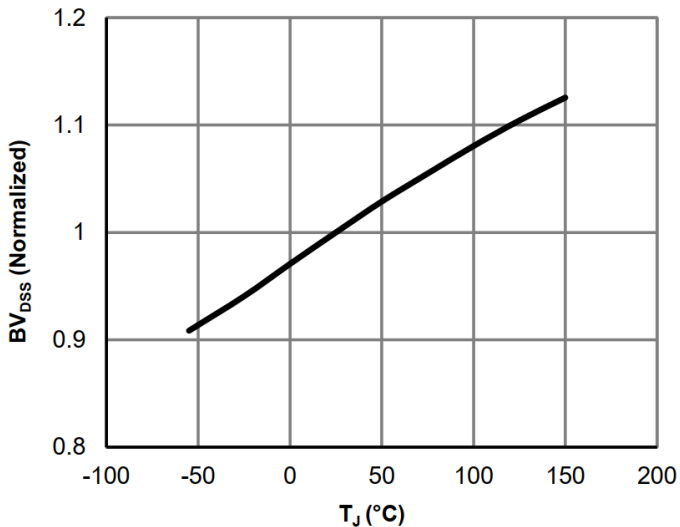
Figure 5: Break Down vs. Junction Temperature
